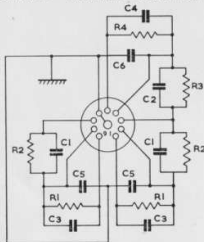
SINGLE LETTER ADAPTOR
