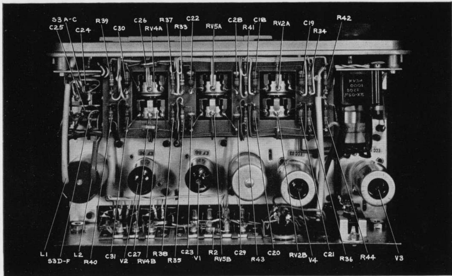
LAYOUT PHOTOGRAPH B
