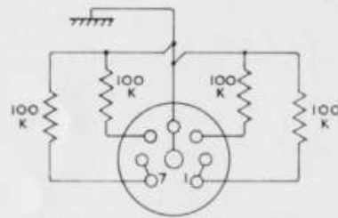
VIEWED FROM INSIDE PLUG
