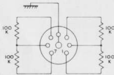
VIEWED FROM INSIDE PLUG
