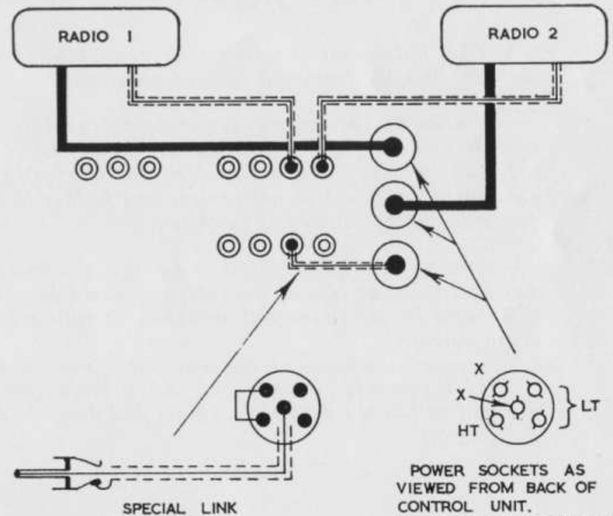
(C) RADIO 2 TO PAIR WITH RADIO 1
