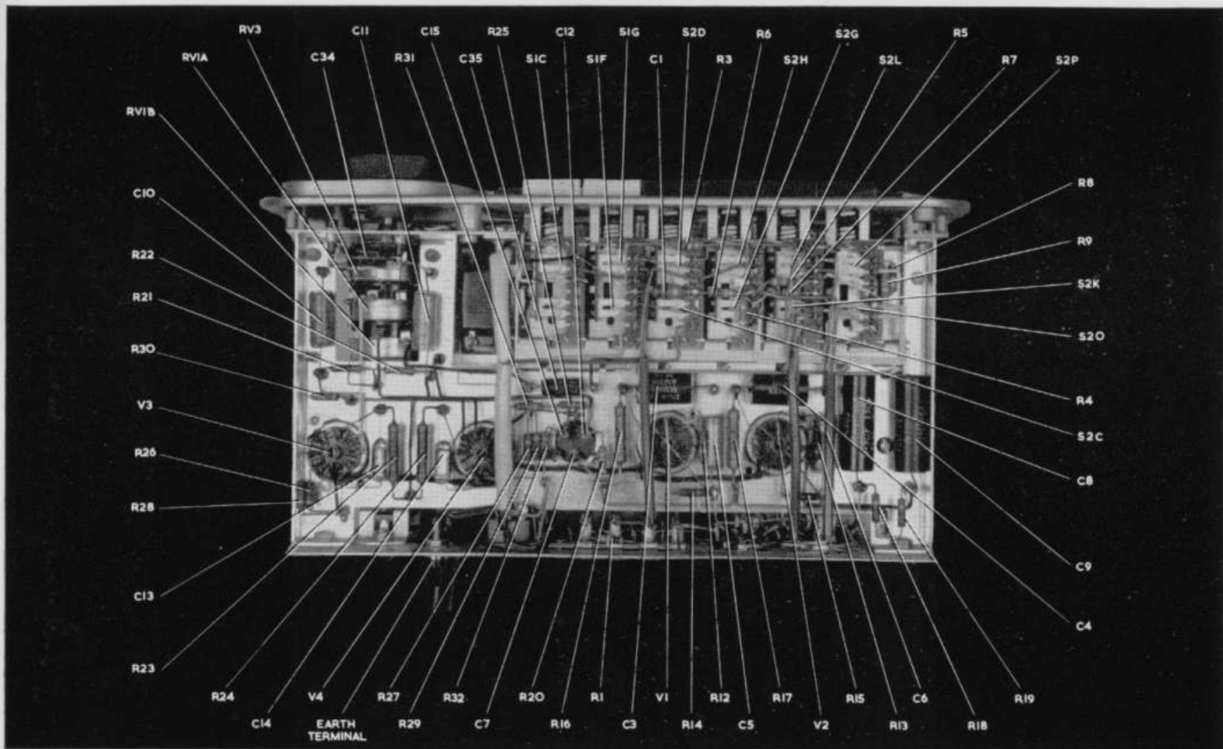
LAYOUT PHOTOGRAPH A
