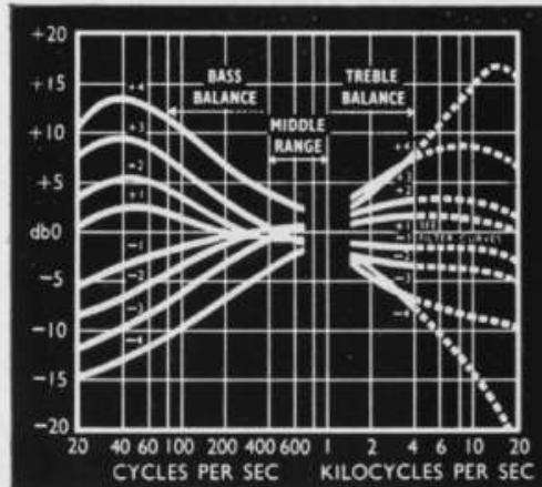
Curves showing (left) effect of bass and treble controls, and (below) extended frequency response and effect of the 7K filter.
