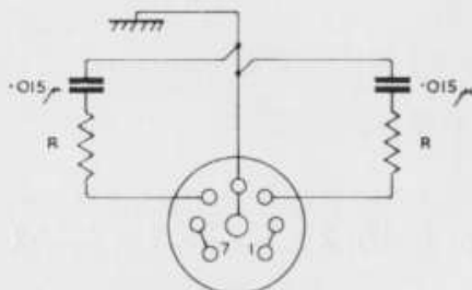
VIEWED FROM INSIDE PLUG
